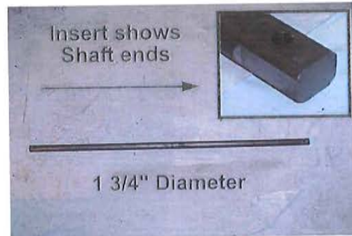
DA Part # : DA- 31033 = 61 inch DA Part # : DA- 33026 = 66 inch CALL FOR ADDITIONAL LENGTHS Description: PINION SHAFTS
