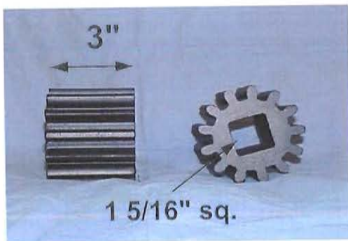
DA Part # : DA- 30304 Ref # : DA-502-SS Description: PINION, STAINLESS STEEL
