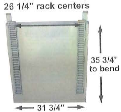
DA Part # : DA- 50289 Ref # : REPLACEMENT Description: DOOR SLIDE ASS'Y Interchange# : MINER
