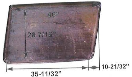
DA Part # : DA- 76031 Ref # : AVAILABLE IN VARIOUS SIZES Description: HOPPER DOOR, TRAP. LH
