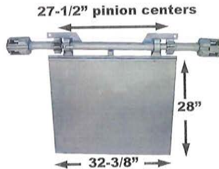
DA Part # : DA- 71140 Ref # : REPLACEMENT Description: DOOR SLIDE ASS'Y Interchange# : KEYSTONE
