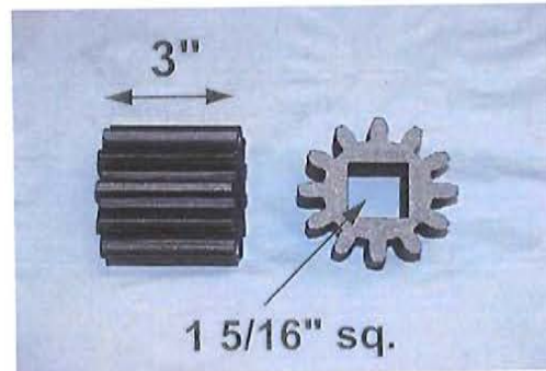
DA Part # : DA- 52082 Ref # : DA-502 Description: PINION GEAR Interchange: Miner
