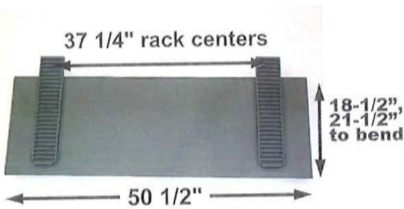
DA Part # : DA- 07118 Ref # : DA-7118 Description: DOOR SLIDE ASSEMBLY Interchange# : MINER
