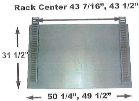
DA Part # : DA- 41329, DA-41328 Ref # : 3CH-429, DA-41328 Description: DOOR SLIDE ASSY
