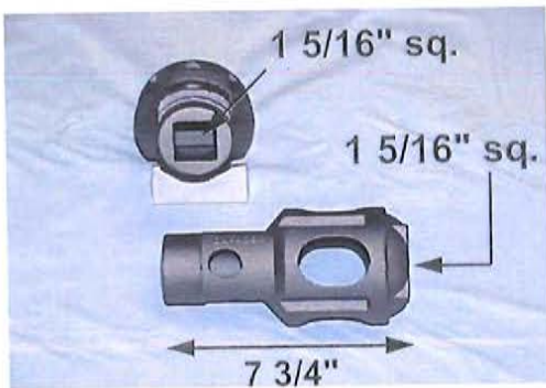
DA Part # : DA- 42391 Ref # : DA-4081 Description: CAPSTAN Interchanges with Miner
