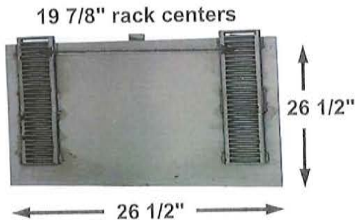
DA Part # : DA- 05804 Ref # : STYLE #4 Description: DOOR SLIDE ASSEMBLY Interchange# : ACF
