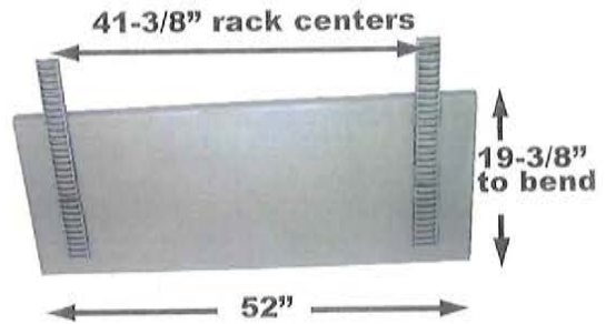
DA Part # : DA- 50210 Ref # : REPLACEMENT Description: DOOR SLIDE ASS'Y Interchange# : MINER
