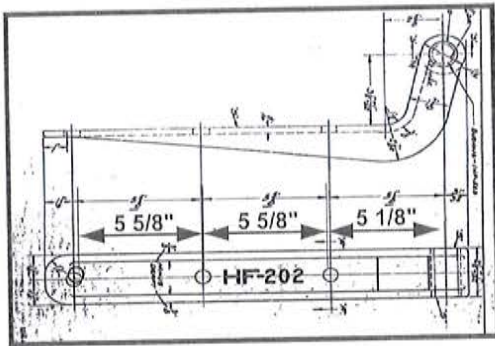
DA Part # : DA- 25202 Ref # : HF-202 Description: HINGE
