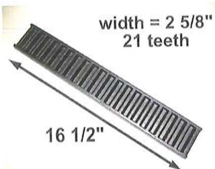
DA Part # : DA-42328 Ref # : DA-7028 Description: RACK Interchange: Miner
