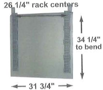
DA Part # : DA- 50287 Ref # : STYLE #1 Description: DOOR SLIDE ASSEMBLY Interchange# : MINER
