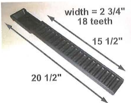
DA Part # : DA- 42340 Ref # : DA-4030 Description: RACK Interchange: Miner
