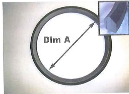
DA Part # : DA- 03654 Ref # : DA-3654-140 Description: BOLSTER RIM REPLACEMENT Dim A = 14"
