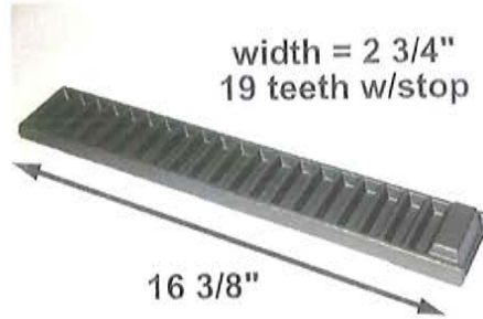
DA Part # : DA- 42339 Ref # : DA-4029 Description: RACK Interchange: Miner
