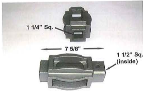
DA Part # DA-01211 Ref # : 2CH-121 Description: CAPSTAN
