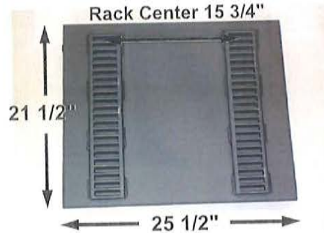
DA Part # : DA- 61294 Ref # : 2CH-654-1 Description: DOOR SLIDE ASSY
