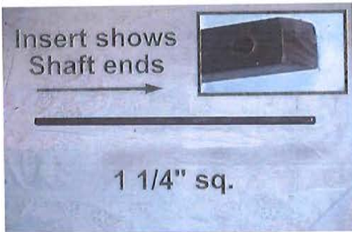
DA Part # : DA-01723 = 36 3/8 inch DA Part # : DA-01733 = 33 inch DA Part # : DA-07248 = 48 inch DA Part # : DA-07177 = 65 inch Description: PINION SHAFT
