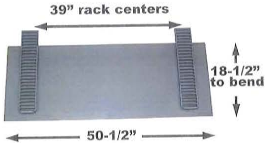
DA Part # : DA- 50209 Ref # : REPLACEMENT Description: DOOR SLIDE ASS'Y Interchange# : MINER
