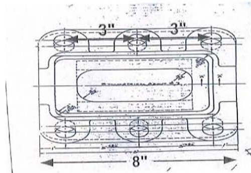
DA Part # : DA- 35350 Ref # : MC-350 Description: CROSSRIDGE FOOT BRACE 33° - 9' BRACE 30° SHEET
