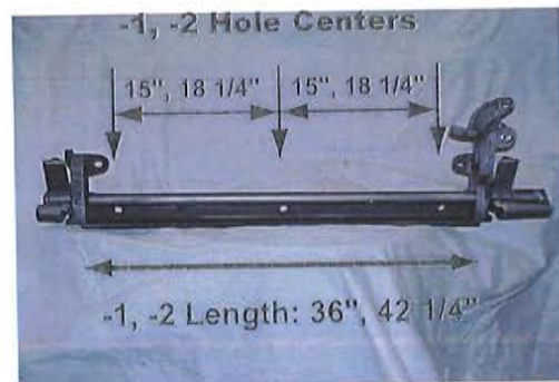
DA Part # : DA- 41611, DA- 41612 Ref # : 4CL-16-1, 4CL-16-2 Description: RH CAM LOCK ASS'Y
