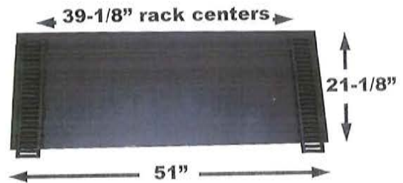
DA Part # : DA-63671 Ref # : WINE Description: DOOR SLIDE ASS'Y
