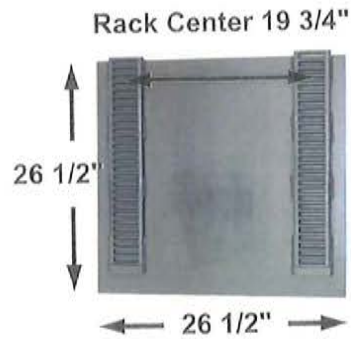
DA Part # : DA- 41254 Ref # : 2CH-404 Description: DOOR SLIDE ASSY
