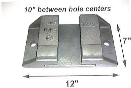
DA Part # : DA- 11222 Ref # : 11222 Description: VIBRATOR BRACKET
