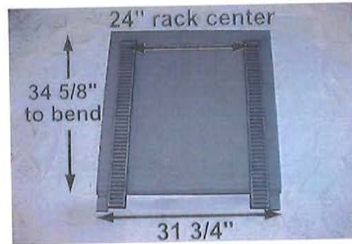
DA Part # : DA- 08410 Ref # : DA-08410 Description: DOOR SLIDE ASSY Interchange: Keystone
