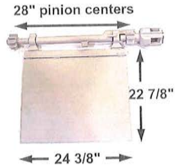
DA Part # : DA- 74510 / DA- 74520 Ref # : AS SHOWN / OPPOSITE Description: DOOR SLIDE ASS'Y Interchange # : KEYSTONE
