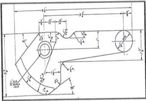
DA Part # : DA- 35323 Ref # : MC-323 Description: HATCH LOCK
