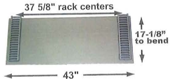
DA Part # : DA- 05765 Ref # : STYLE #5 Description: DOOR SLIDE ASSEMBLY Interchange# : ACF
