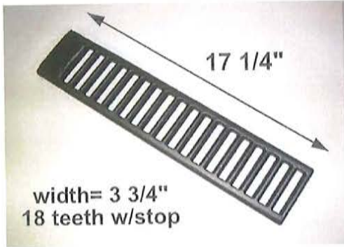
DA Part # : DA- 13096 Ref # : 2CH-156 Description: RACK
