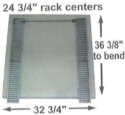
DA Part # : DA- 07118 Ref # : DA-7118 Description: DOOR SLIDE ASSEMBLY Interchange# : MINER
