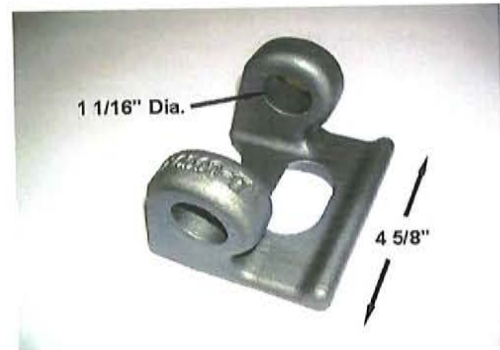
DA Part # : DA- 50017 Ref # : Description: HINGE BUTT Interchange: Rapid Discharge Car
