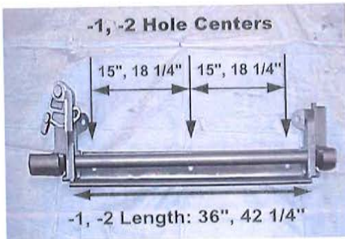
DA Part # : DA- 41511, DA- 41512 Ref # : 4CL-15-1, 4CL-15-2 Description: LH CAM LOCK ASS'Y
