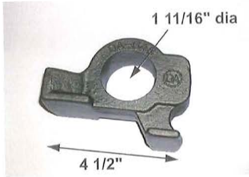
DA Part # : DA- 00648 Ref # : DA-648 Description: BEARING BLOCK Interchanges with Keystone
