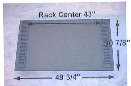
DA Part # : DA- 31313 Ref # : 3CH-303 Description: DOOR SLIDE ASSY
