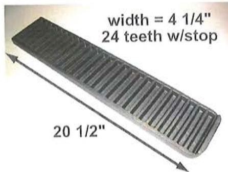
DA Part # : DA- 42372 Ref # : DA-422 Description: RACK Interchange: Miner
