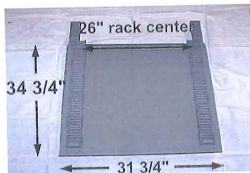
DA Part # : DA- 07987 Ref # : DA-7987 Description: DOOR SLIDE ASSEMBLY Interchange#: MINER
