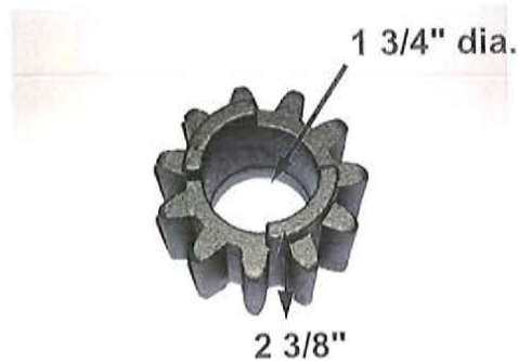
DA Part # : DA- 21129, DA- 21130 Ref # : 2CH-29, DA-29-304-SS Description: PINION, CARBON, S.S.
