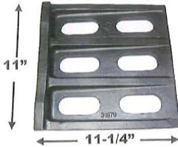
DA Part # : DA- 81777 Ref # : 578106-0 Description: DRAFT LUG, FRONT Interchange:
