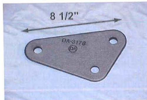
DA Part # : DA- 31780 w/ 13/16" holes Ref # : DA-3178 Description: FILLER
