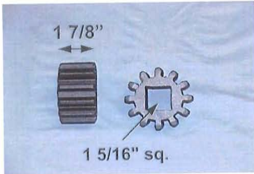
DA Part # : DA- 70209 Ref # : DA-29 Description: PINION GEAR Interchange: Miner
