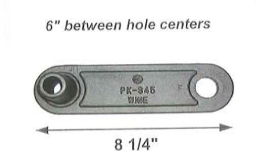
DA Part # : DA-37345 Ref # : PK-345 Description: TRUNNION WASHER
